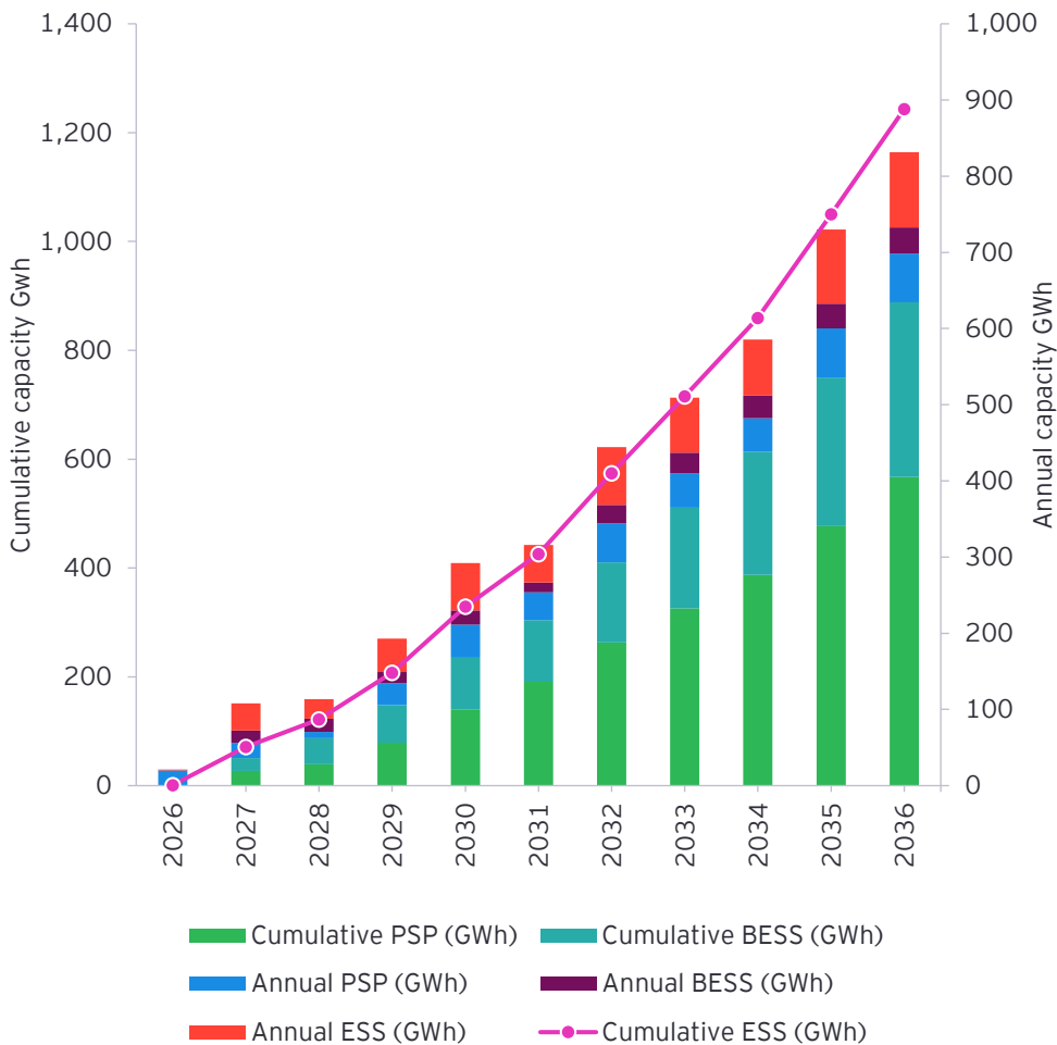
Annual BESS capacity addition projection 2026-2036
