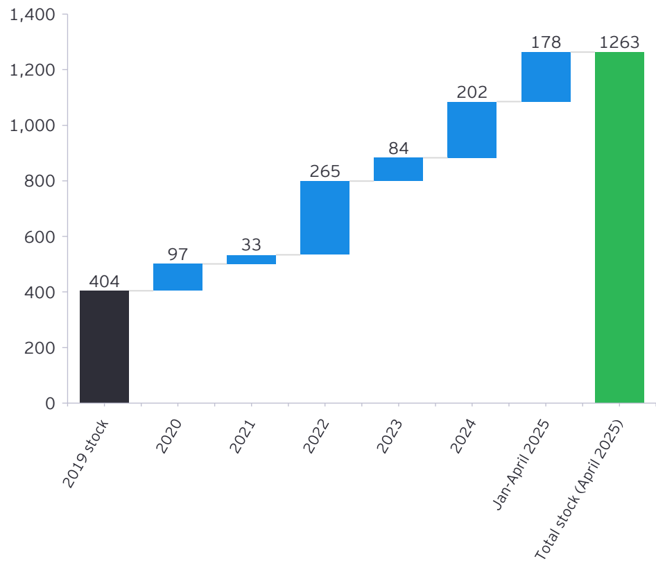
Trends in DC capacity/supply addition in MW across top seven Indian cities
